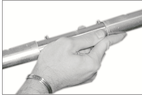
Figure 2: Place steel connector into two steel bars.
